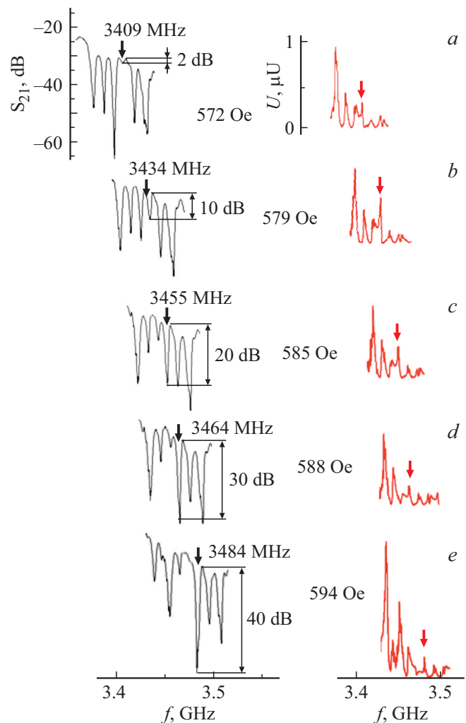
Figure 2. The dependency plots are S_{21}(f) (black curves) and U(f) (red curves) at H = 572, 579, 585, 588 and 594 Oe ( a, b, c, d, e , respectively). The vertical scale range in all figures is the same.
