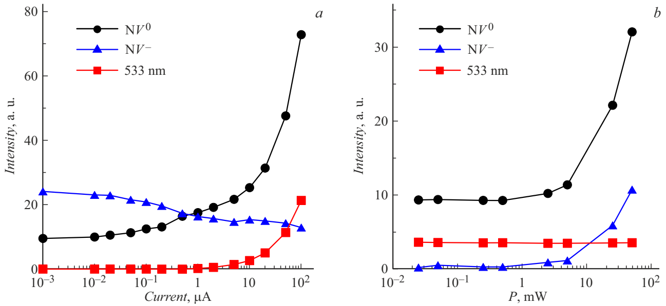
Figure 3. Dependences of luminescence intensity with combined photoexcitation and electrical excitation on the level of current (laser power, 50 mW; wavelength, 514 nm) (a) and laser power (diode current, 20 \mu\text{A} ) (b).
