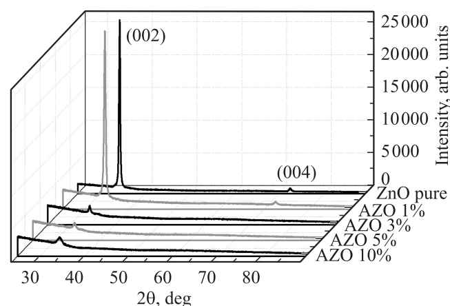
Figure 2. X-ray diffraction patterns of AZO films grown by 5 cycle spin-coating.
