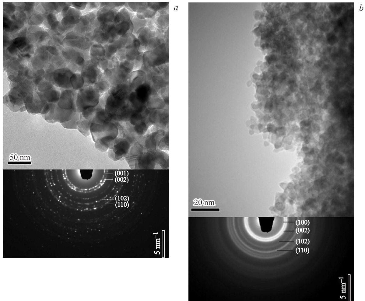
Figure 3. TEM images and the selected-area electron diffraction pattern of: a — pure ZnO nanoparticles, b — AZO 10% nanocomposite, elaborated by spin coating.
