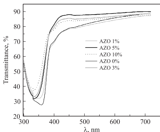
Figure 4. Optical transmittance spectra of ZnO and AZO thin films prepared by spin-coating (5 layers) deposited at glass substrate.
