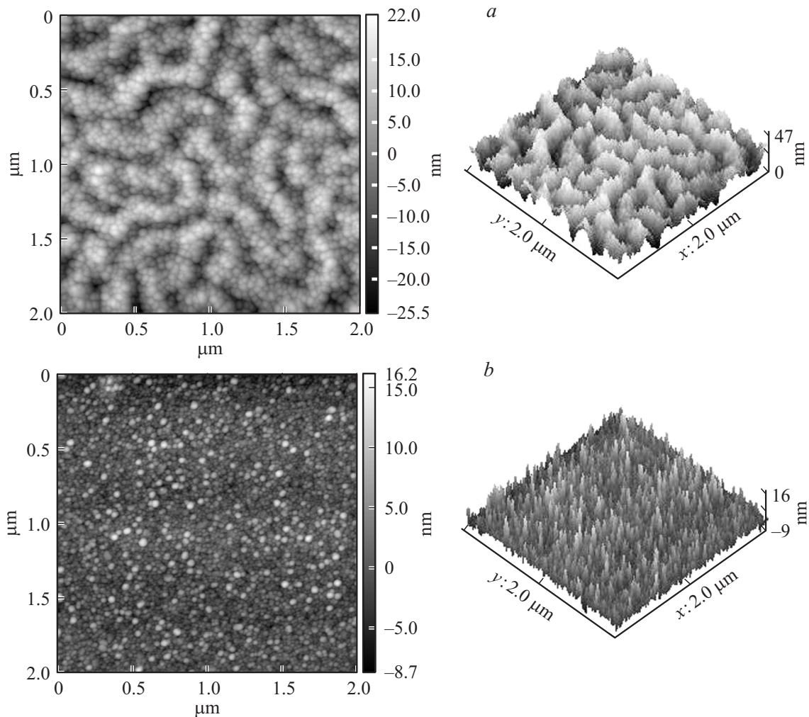
Figure 1. The 2D and 3D AFM micrographs of: a — pure ZnO film annealed at 450°C for 1 h in air. b — AZO film annealed at 450°C for 1 h in air, with concentration of 5 at%.
