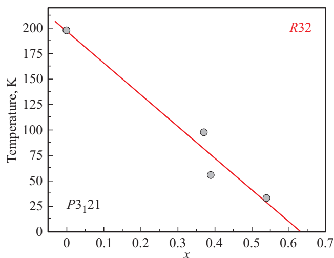
Figure 6. Phase diagram: temperature of structural transition in solid solutions TbFe_{3-x}Ga_x(BO_3)_4 vs gallium content.
