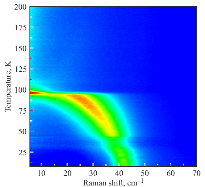
Figure 4. Intensity map at low frequencies in \text{TbFe}_{2.45}\text{Ga}_{0.55}(\text{BO}_3)_4 crystal (by embedding).
