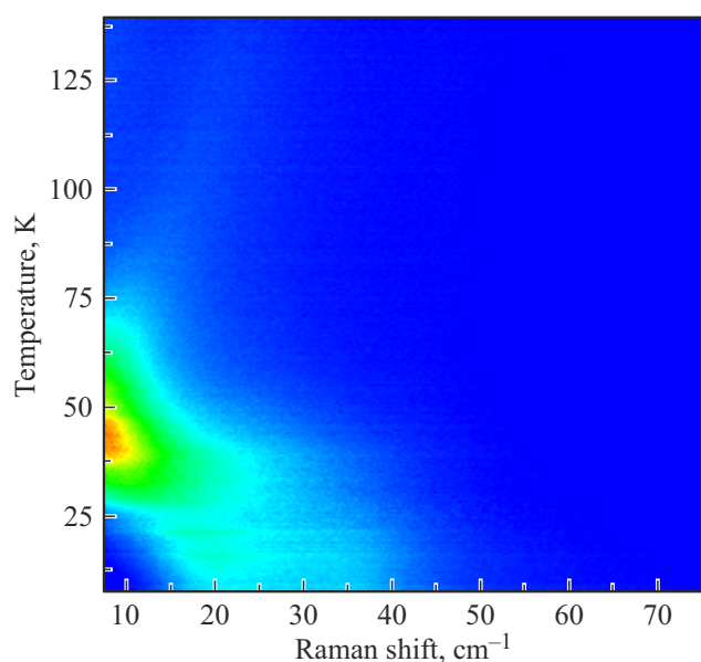
Figure 5. Intensity map at low frequencies in TbFe_{2.4}Ga_{0.6}(BO_3)_4 crystal (by embedding). The structural transition temperature (56 K) is presumably close to the magnetic transition temperature (not yet determined) of the solid solution.
