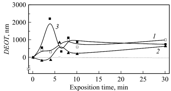
Figure 6. Dependences of the PAAO+Ag membrane effective optical thickness on the time of gas puffing into the measuring chamber at wavelengths of 650 nm (1), 750 nm (2), 850 nm (3).
