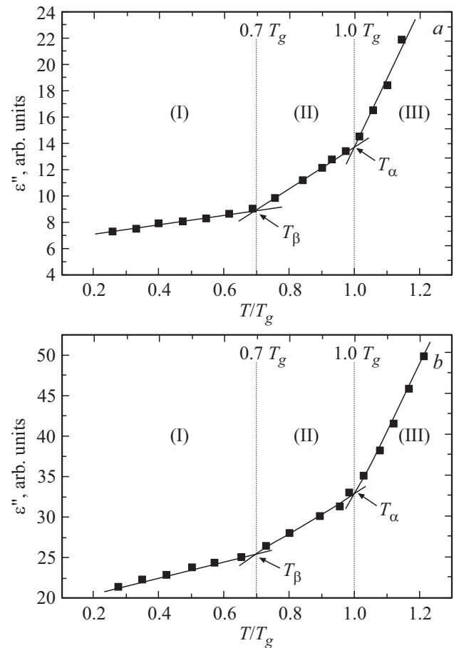
Figure 3. Dielectric losses \epsilon''(T/T_g) at the frequencies of 0.43 THz for polyvinylchloride ( a ) and \nu = 0.54 THz for polyamide PA-6 ( b ). The solid lines show the linear approximation of dependence \epsilon''(T/T_g) in modes (I), (II) and (III). T_\beta and T_\alpha are the points of intersection of linear approximation (I) with (II) and (II) with (III), respectively.
