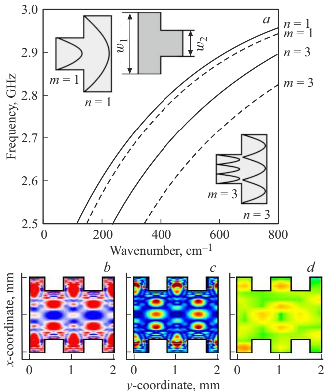
Figure 4. Dispersions of the first and third width modes for ferrite microwave guides with the width w_1 = 353 \mu\text{m} and w_2 = 233 \mu\text{m} (a). The result of calculating dynamic magnetization at a distance of 1.2 mm from the input antenna in the form of maps of the spatial distribution of the magnetization component m_z (b), intensity I(y, z) (c) and an experimental map of the integrated intensity distribution I(y, z) MSV (d).
