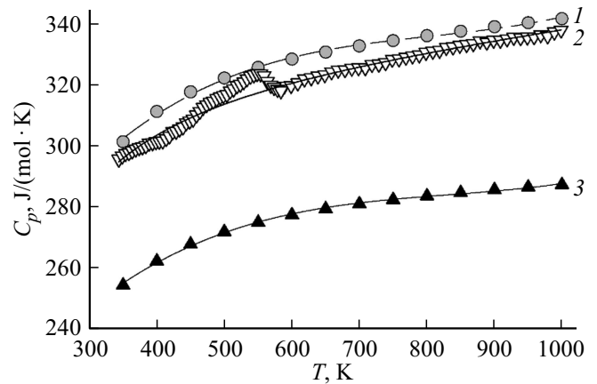
Figure 3. Temperature dependence of heat capacity of \text{CuEu}_2\text{Ge}_2\text{O}_8 (1, 2) and \text{Eu}_2\text{Ge}_2\text{O}_7 (3). 1 — the data calculated according to Neumann–Kopp, 2 — the experiment.
