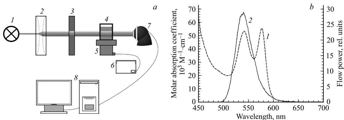
Figure 1. (a) Scheme of setup for registration of erythrocytes agglutination reaction: 1 — LED, 2 — condenser, 3 — neutral light filter, 4 — cuvet, 5 — ultrasonic converter, 6 — ultrasonic generator, 7 — eight-bit digital photo camera, 8 — computer. (b) Spectra: 1 — hemoglobin absorption (left ordinate axis), 2 — LED radiation (right ordinate axis).
