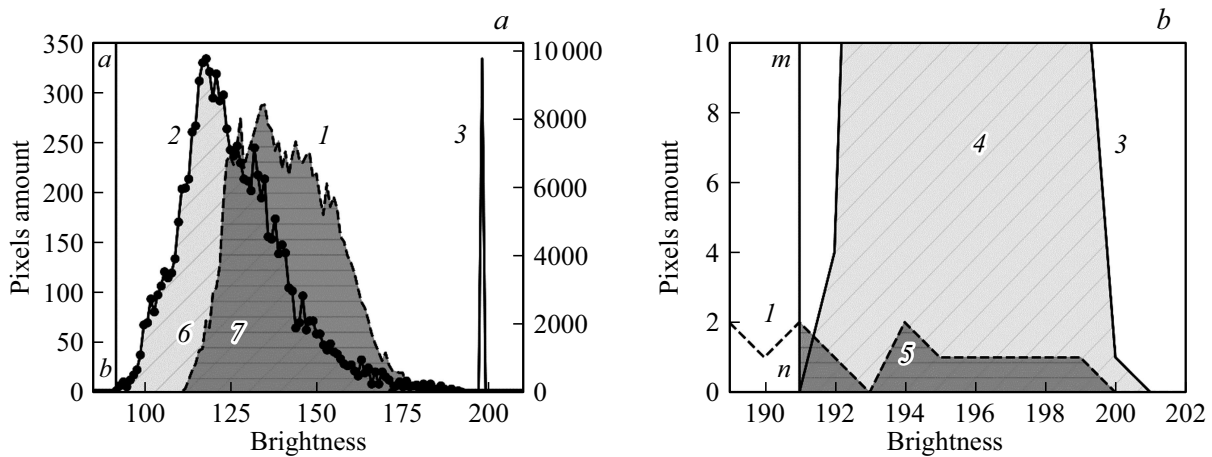
Figure 4. (a) Photo images pixels distribution by brightness: 1 — „pure“ sample, 2 — negative agglutination reaction, 3 — positive agglutination reaction. Curves 1, 2 — left ordinate axis, 3 — right ordinate axis, ab — boundary value line ( B_{bound} ) for pair of „pure sample“–negative reaction“, 6 and 7 — parts of areas of pixels distribution for negative reaction of RBC agglutination S_- and „pure“ sample S_0 respectively if B \geq B_{bound} for both cases. (b) Magnified image of the fragment of the same distribution (fig. 4, a) for „pure“ sample (1) and positive reaction (3), mn — boundary value line ( B_{bound} ) for pair of „pure sample“–positive reaction“, 4 and 5 — parts of areas of pixels distribution for positive reaction of RBC agglutination S_+ of pure sample S'_0 respectively if B \geq B_{bound} for both cases.
