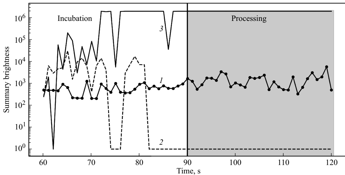
Figure 6. Dependences of summary pixels brightness on observation time: 1 — S_{N0} , 2 — S_{Na} , 3 — S_{Nb} .
