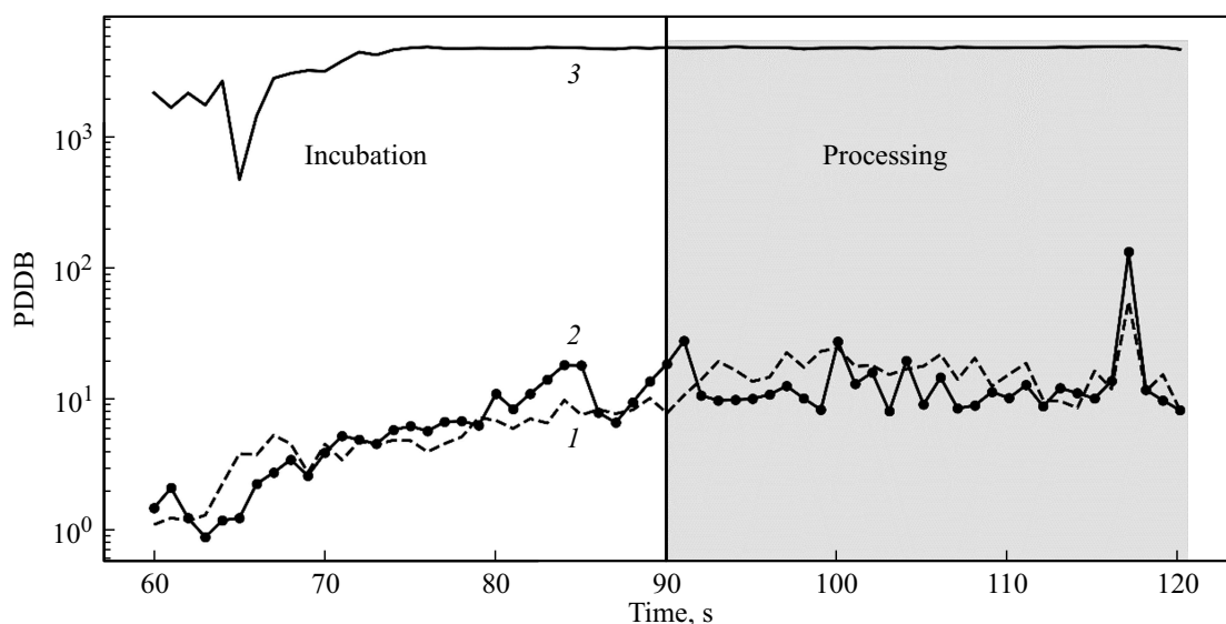
Figure 7. Dependences of pixels distribution density by brightness PDDB in the zone W on observation time: 1 — PDDB 0 , 2 — PDDB a , 3 — PDDB b .
