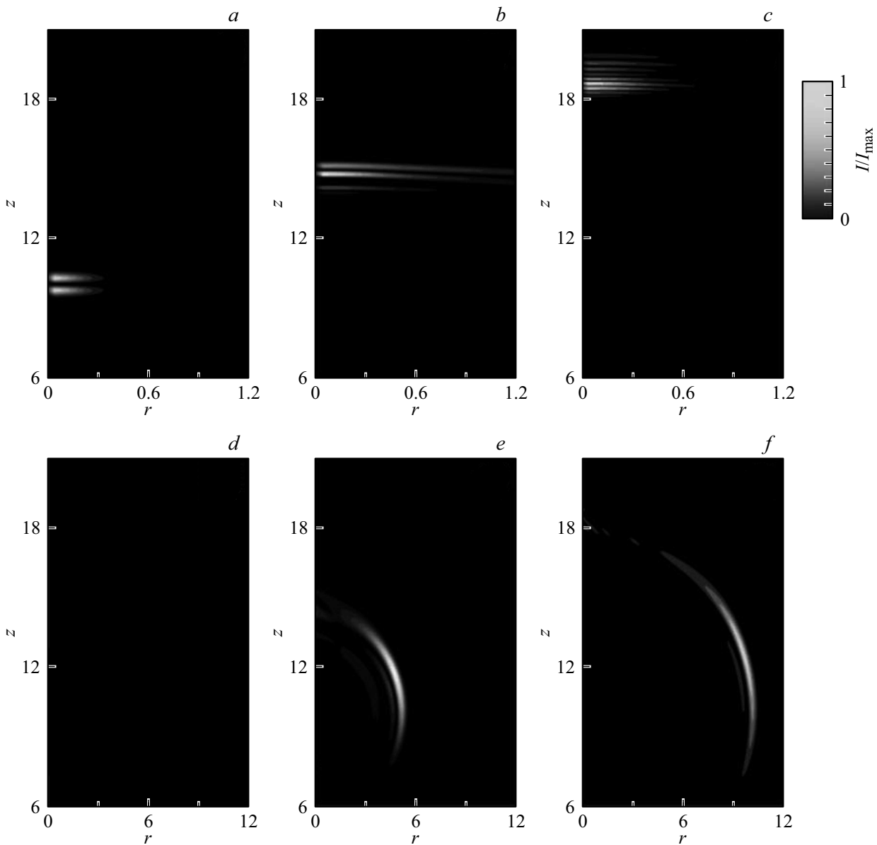
Figure 1. The intensity for x-component of the field ( a-c ) and for y-component ( d-f ) as function of coordinates: ( a, d ) t = 0 ; ( b, e ) t = 5 \cdot 10^{-14} s; ( c, f ) t = 10^{-13} s. I_{\max} is the maximum intensity for each moment of time. Units along r and z axes correspond to 2 \cdot 10^{-5} m.
