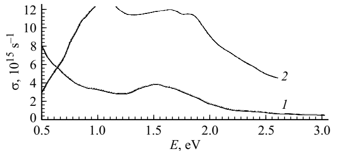
Figure 2. Optical conductivity spectrum of aluminum ( T = 298 \text{ K} ): 1 is aluminum film, 2 is spectrum of pressed ASD-4 powder.
