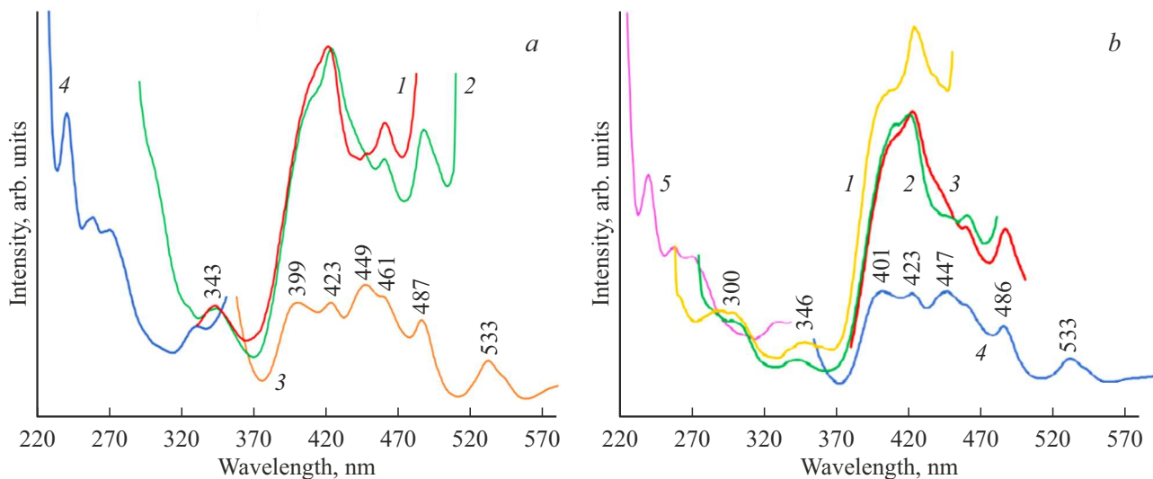
Figure 3. Photoluminescence and luminescence excitation spectra of the sample 1 ( a , curves 1–3 and curve 4, respectively) and the sample 5 ( b , curves 1–4 and curve 5 respectively). Luminescence excitation wavelength 257 (curves 1); 270 (curves 2); 330 (Fig. a , curve 3), 350 (Fig. b , curve 3), 390 nm (Fig. b , curve 4). Recording wavelength at measuring excitation spectra 390 nm
