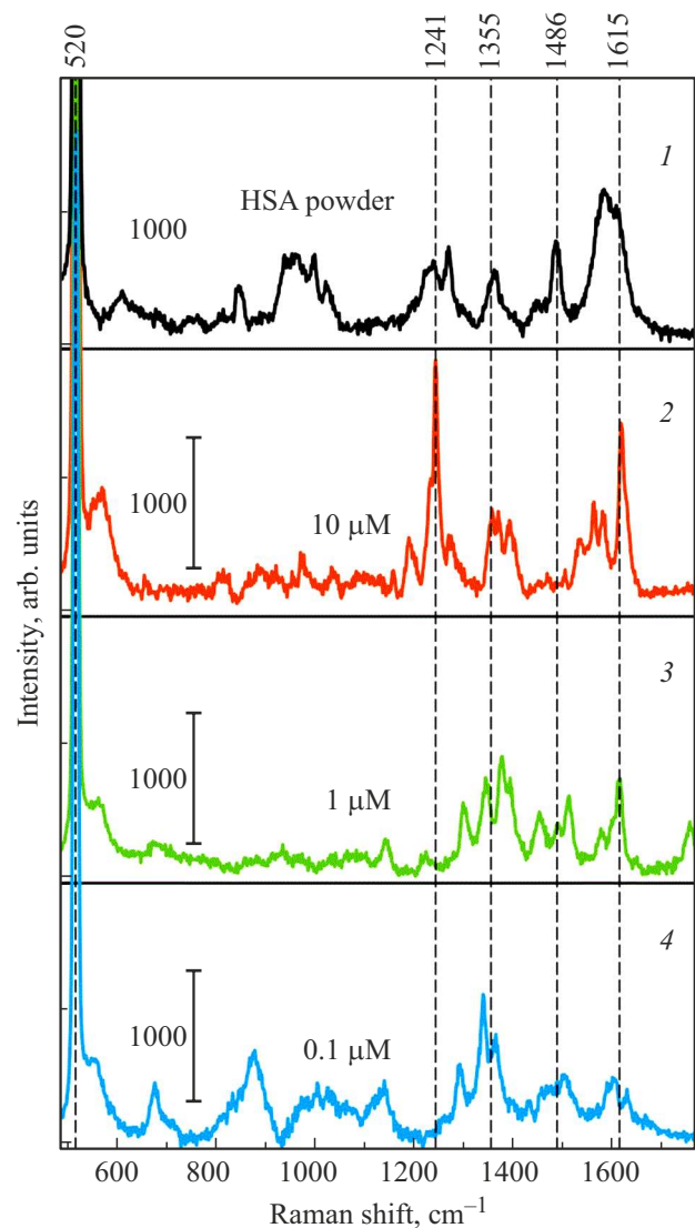
Figure 2. RS spectrum of HSA powder on a single-crystal silicon wafer ( 1 ); SERS spectra of HSA adsorbed on AgSNW with different concentrations: 10 ( 2 ), 1 ( 3 ) and 0.1 \mu\text{M} ( 4 ).
