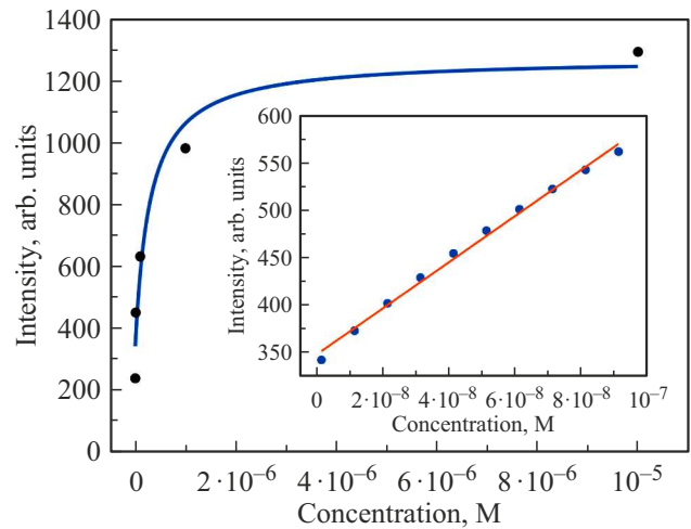
Figure 4. Dependence of the intensity of the SERS peak of amide I at frequency of 1618 cm -1 on the concentration of the InIB protein. The blue line shows the result of approximation by the Langmuir adsorption isotherm. The inset shows the first 10 points obtained from the Langmuir isotherm at low concentrations of the InIB protein and the result of their approximation (red line) by the least squares method.
