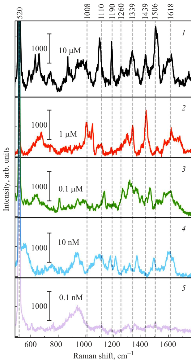
Figure 3. SERS spectra of the InIB protein adsorbed on AgKHN with a concentration of 10 (1), 1 (2), 0.1 μM (3) and 10 (4), 1 nM (5).
