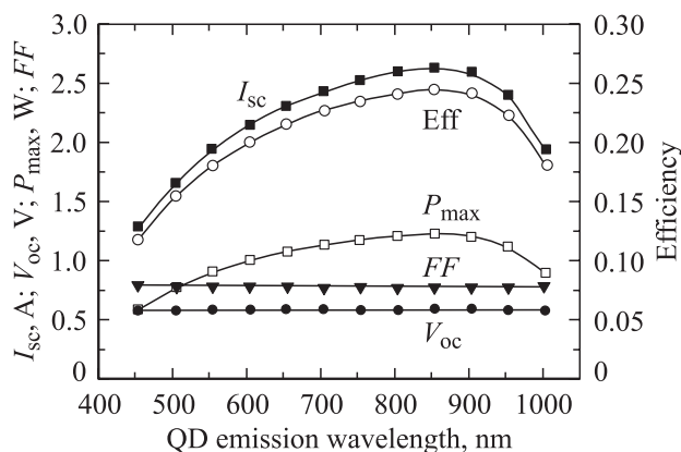
Figure 5. Effect of small-band QD emission ( 500 \text{ W/m}^2 ) on the parameters I_{sc} , V_{oc} , FF , P_{max} , and efficiency (Eff) of the mc-Si solar cell as a function of center emission wavelength. Left-hand scale: I_{sc} , V_{oc} , and P_{max} ; right-hand scale — efficiency.
