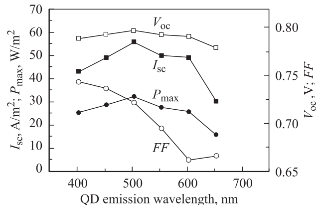
Figure 6. Effect of small-band QD emission ( 500 \text{ W/m}^2 ) on the parameters I_{sc} , V_{oc} , FF , and P_{max} of the a-Si:H solar cell as a function of center emission wavelength. Left-hand scale: I_{sc} and P_{max} , right-hand scale: V_{oc} and FF .
