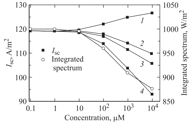
Figure 9. Short-circuit current I_{sc} of the a-Si:H solar cell as a function of QD concentration for combinations of the quantum efficiency \eta_e and capture efficiency \eta_t : 1 — \eta_e = 1 , \eta_t = 1 , 2 — \eta_e = 0.8 , \eta_t = 1 , 3 — \eta_e = 1 , \eta_t = 0.75 , and 4 — \eta_e = 0.8 , \eta_t = 0.75 . The integrated spectrum is shown to the right-hand scale for \eta_e = 0.8 , \eta_t = 0.75 .
