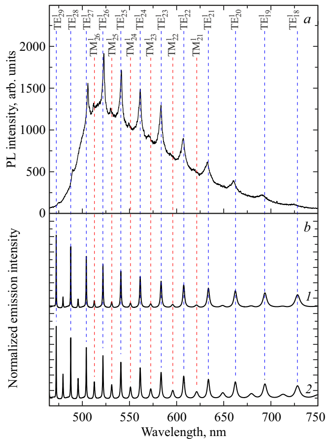
Figure 2. a ) Experimental PL spectrum of the hybrid spherical microresonator with FITC. The excitation wavelength is \lambda = 442 nm. Vertical dashed lines show the specified WGM positions. b ) Calculated emission spectrum of HSMR–FITC, 1 — emitting dipoles are oriented parallel to the surface, 2 — emitting dipoles are oriented in all directions with the equal probability.
