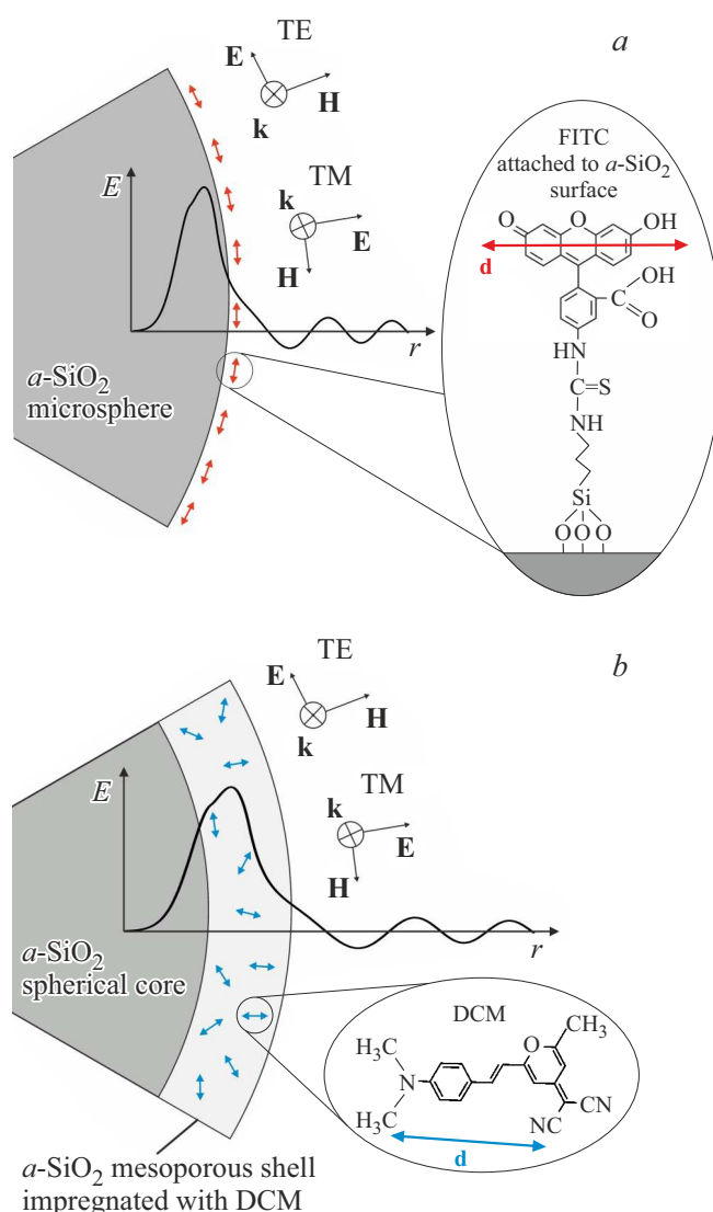
Figure 1. Schematic diagram of a cross-section segment a ) HSMR–FITC and b ) HSMR–DCM. Small double-headed arrows near the microsphere surface ( a ) and inside the shell ( b ) show the emitting dipole moment orientation of the FITC ( a ) and DCM ( b ) molecules. Details: structure of the FITC molecule attached to the microsphere surface ( a ), DCM molecule in pores ( b ) and orientation of dipole emitting moment vector d of these molecules. Both figures show electric field vectors E , magnetic field vectors H and wave vector k for TE- and TM-polarized WGM and a curve showing typical distribution of electric field strength E over the radial coordinate r for TE-polarized WGM with q = 1 .
