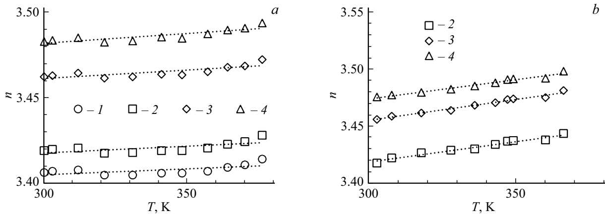
Figure 2. Dependences of changes in the refraction index of samples № 1 (a) and № 2 (b) at frequencies \nu = 0.5 (1), 0.7 (2), 1.0 (3), 1.1 THz (4) on temperature.
