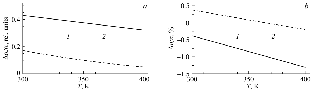
Figure 3. Dependences of changes in absorption coefficient (a) and refraction index (b) of sample 1 relative to sample 2 at frequencies 0.7 (1) and 1.1 THz (2) on temperature.
