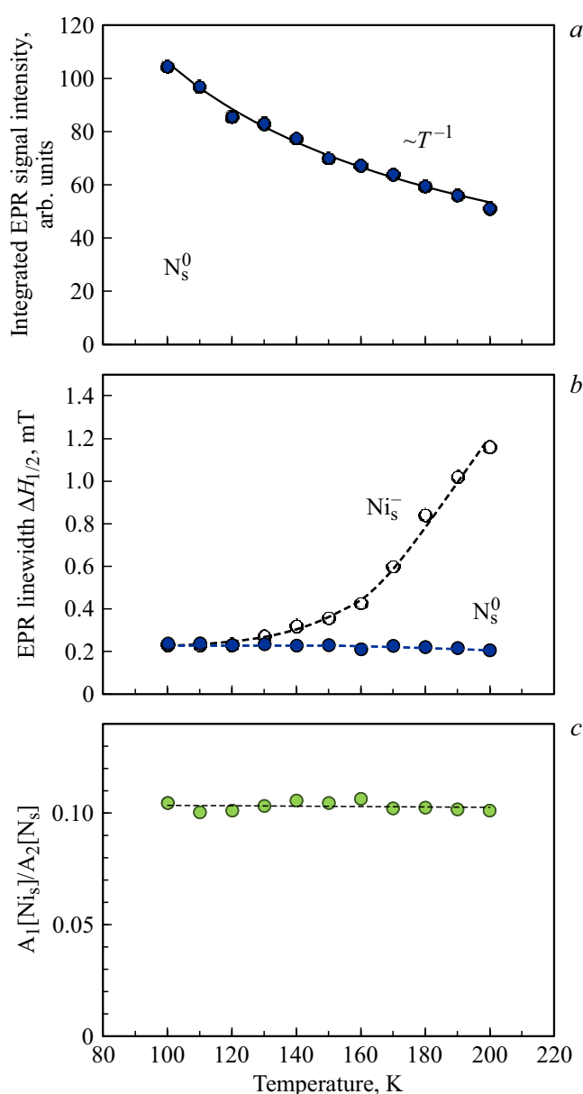
Figure 5. Temperature dependences of EPR signal parameters: (a) integral signal intensity for N_S^0 , (b) \Delta H_{1/2} linewidth for centers N_S^0 and Ni_S^- , and (c) ratio of integral signal intensities for centers Ni_S^- and N_S^0 . Microwave power — 1 \mu W and frequency — 9.081 \text{ GHz} .
