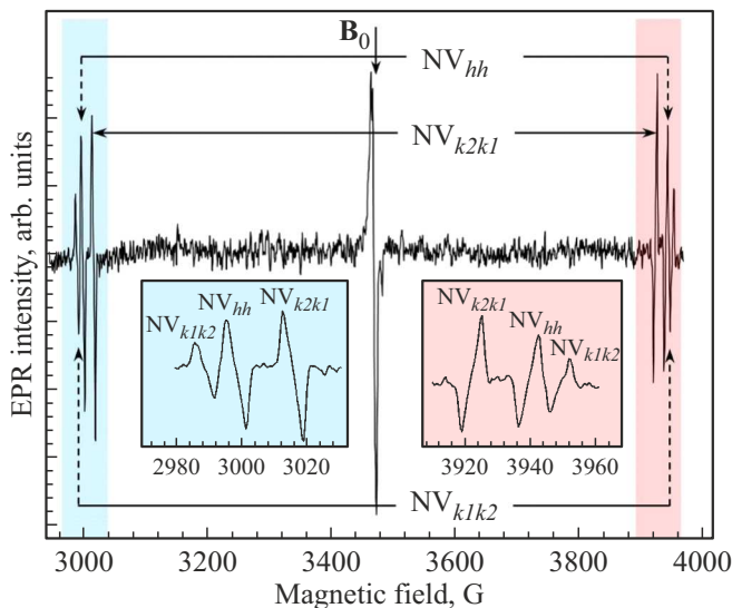
Figure 2. The EPR spectrum of the sample of 6H\text{-}^{28}\text{SiC} irradiated with electrons and annealed at 900^\circ\text{C} , recorded with magnetic field modulation 5 G, temperature T = 150\text{ K} and laser excitation \lambda = 980\text{ nm} . The orientation of the magnetic field \mathbf{B} \parallel \mathbf{c} . The resonant magnetic fields corresponding to the permitted transitions between the spin sublevels of triplet centers, shown in the inserts on an enlarged scale, are designated as \text{NV}_{hh} , \text{NV}_{k2k1} and \text{NV}_{k1k2} . The colors show the enhanced absorption and radiation of microwaves, in accordance with the diagram of triplet sublevels in Figure 1. The magnetic field \mathbf{B}_0 , corresponding to the center of mass of the triplet spectra ( g -factor g = 2.00 ), is shown by a vertical arrow.
