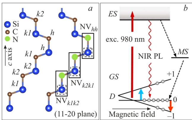
Figure 1. (a) View of the lattice 6H-SiC in the plane (11–20). Hexagonal ( h ) and quasi-cubic ( k1 , k2 ) non-equivalent positions are indicated respectively. Silicon vacancies are shown by dotted lines, and paired NV-defects are marked by rectangles. (b) The energy structure of the optical pumping cycle of the spin sublevel m_s = 0 of the main ( GS ) triplet state of S = 1 NV-centers. The dotted arrows show spin-dependent recombination from the excited state ( ES ) to GS through the metastable state ( MS ) under the action of optical excitation ( \lambda = 980 nm). Spin-dependent luminescence is designated as NIR PL. The separation of spin sublevels in the absence of a magnetic field is indicated by the fine structure parameter D . The external magnetic field causes the Zeeman splitting of the ground state. The vertical arrows show the allowed EPR transitions between the spin sublevels of the triplet.
