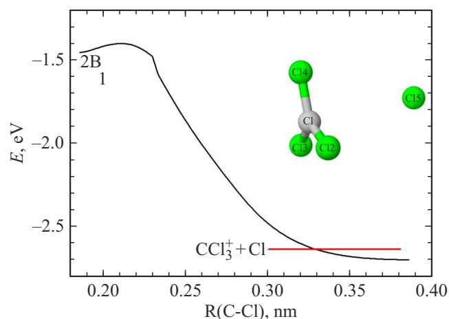
Figure 2. Dependence of the relative energy of the molecular ion of \text{CCl}_4^+ along the path of the chlorine atom separation reaction. The energy reference point is the total energy of the \text{CCl}_4^+ ion in the optimal geometry of the neutral molecule. A straight red line is the energy effect of the reaction.
