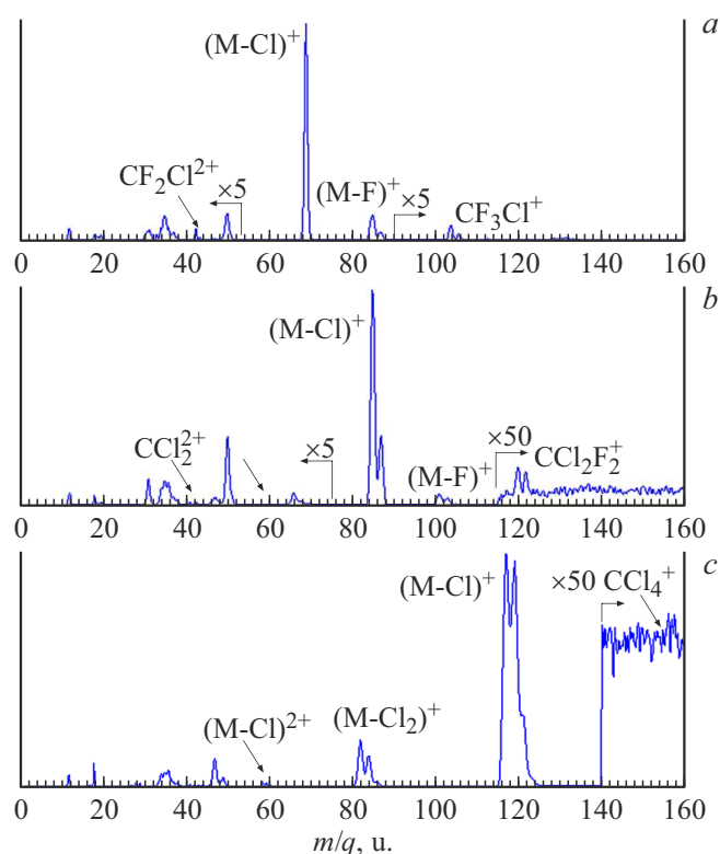
Figure 1. Mass spectra of ion fragments formed in the process of capture of one electron by \text{He}^{2+} ions from halogenomethane molecules: a — \text{CF}_3\text{Cl} , b — \text{CCl}_2\text{F}_2 , c — \text{CCl}_4 .
