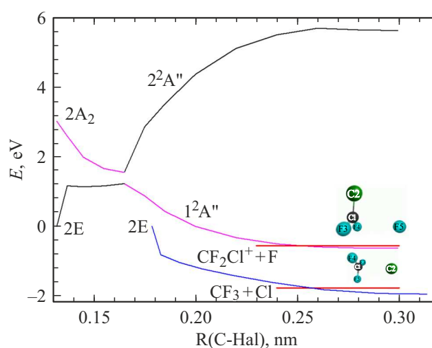
Figure 4. Dependence of the relative energy of the molecular ion of \text{CF}_3\text{Cl}^+ along the path of the halogen atom separation reaction (Cl or F). The energy reference point is the total energy of the \text{CF}_3\text{Cl}^+ ion in the optimal geometry of the neutral molecule. Straight red lines — the energy effect of the reaction.
