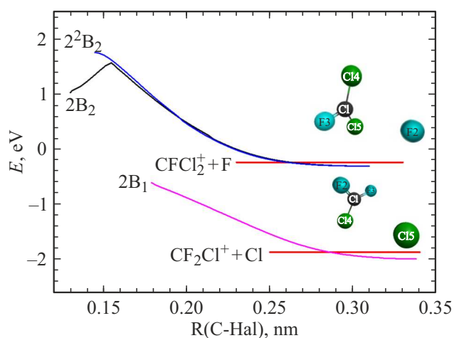
Figure 3. Dependence of the relative energy of the molecular ion \text{CF}_2\text{Cl}_2^+ along the path of the halogen atom separation reaction (Cl or F). Energy reference point is the total energy of the \text{CF}_2\text{Cl}_2^+ ion in the optimal geometry of a neutral molecule. Straight red lines — the energy effect of the reaction.
