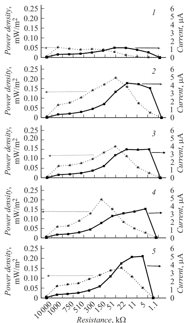
Figure 4. Dependence of BES power on the connected load: 1 — BES-K, 2 — BES-R, 3 — BES-HA, 4 — BES-HAu, 5 — BES-HAl.
