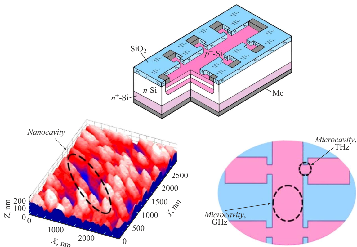
Figure 1. A silicon nanosandwich structure possessing nano- (on the surface of p^+ -Si) and microresonators tuned to selected wavelengths of the spectral range, and used as an IR emitter with THz modulation. The image of the surface p^+ -Si was obtained by scanning tunneling microscopy (STM).
